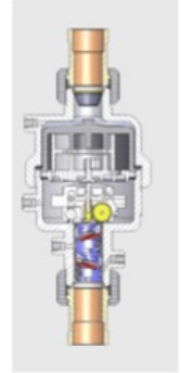
Patented Testable Plastic Water Meter (Zero Lead)
